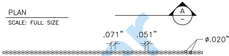
A SECTION SCALE: FULL SIZE
