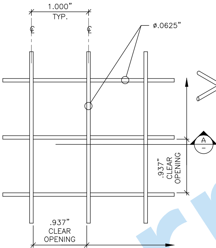
PLAN SCALE: FULL SIZE
