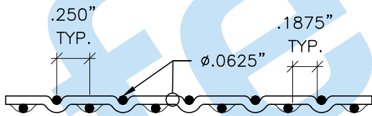
A SECTION SCALE: FULL SIZE
